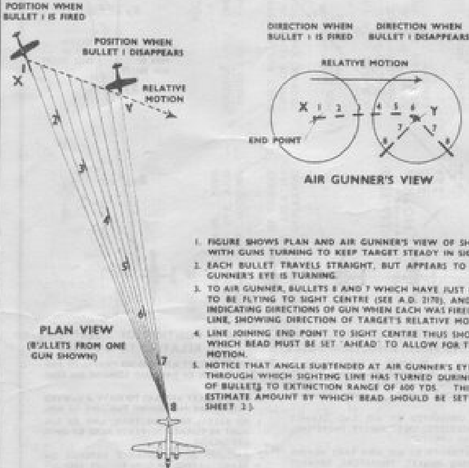
FIG. B—TRACER PATTERN, GUNS TURNING
