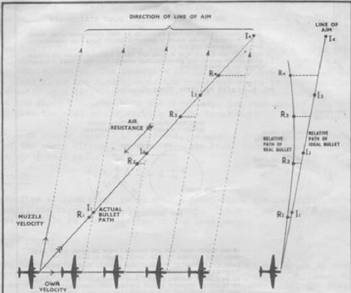
FIG. A-SUCCESSIVE POSITIONS OF IDEAL AND REAL BULLETS FIRED SIMULTANEOUSLY
